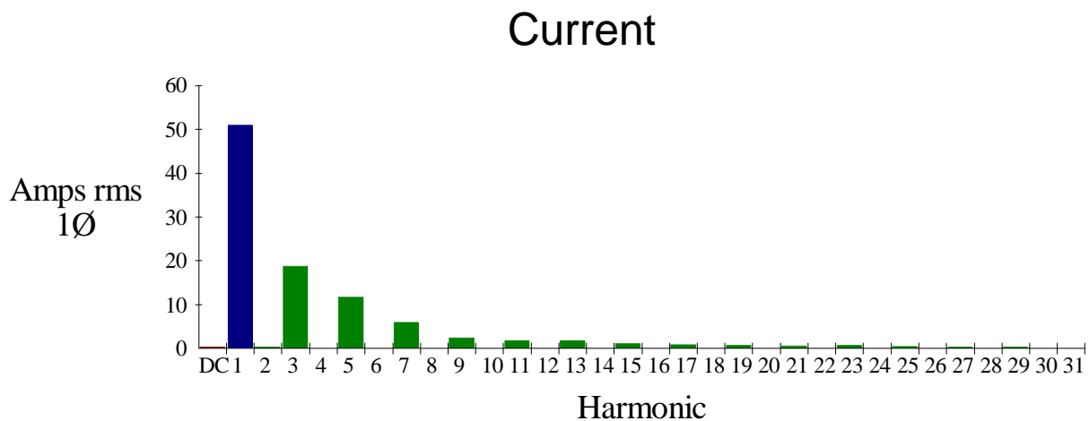
Graph 3 & 4 - Existing Xfmr Secondary Current Waveform and Harmonic Spectrum
